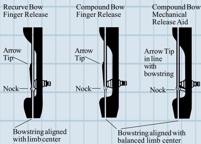
Fig. 7 - Arrow Centering
